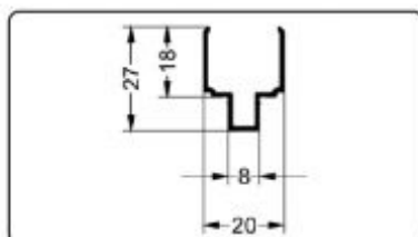
Isolerglasadapter R119
