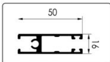
Topp/botten R102
